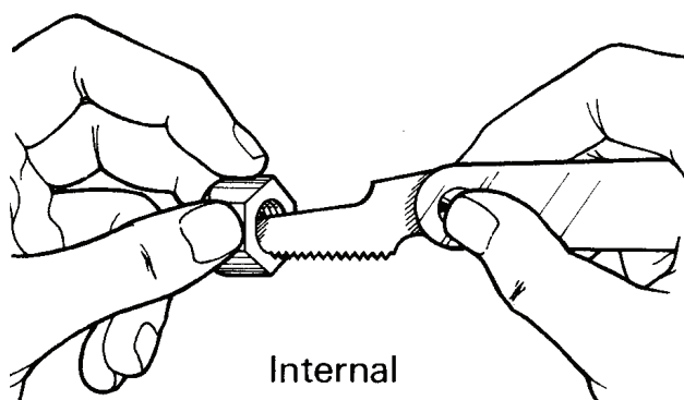
Internal USE OF SCREW PITCH GAUGES
