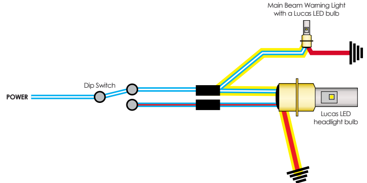
Power Flow With A Lucas LED Bulb Fitted To The Main Beam Warning Light
